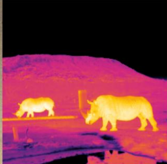
ASTRO-ECOLOGY
