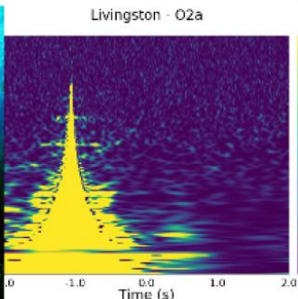
GRAVITY SPY
