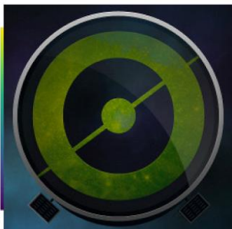
GALAXY ZOO
